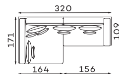
NAROŻNIK SET 4 CORNER SET 4
